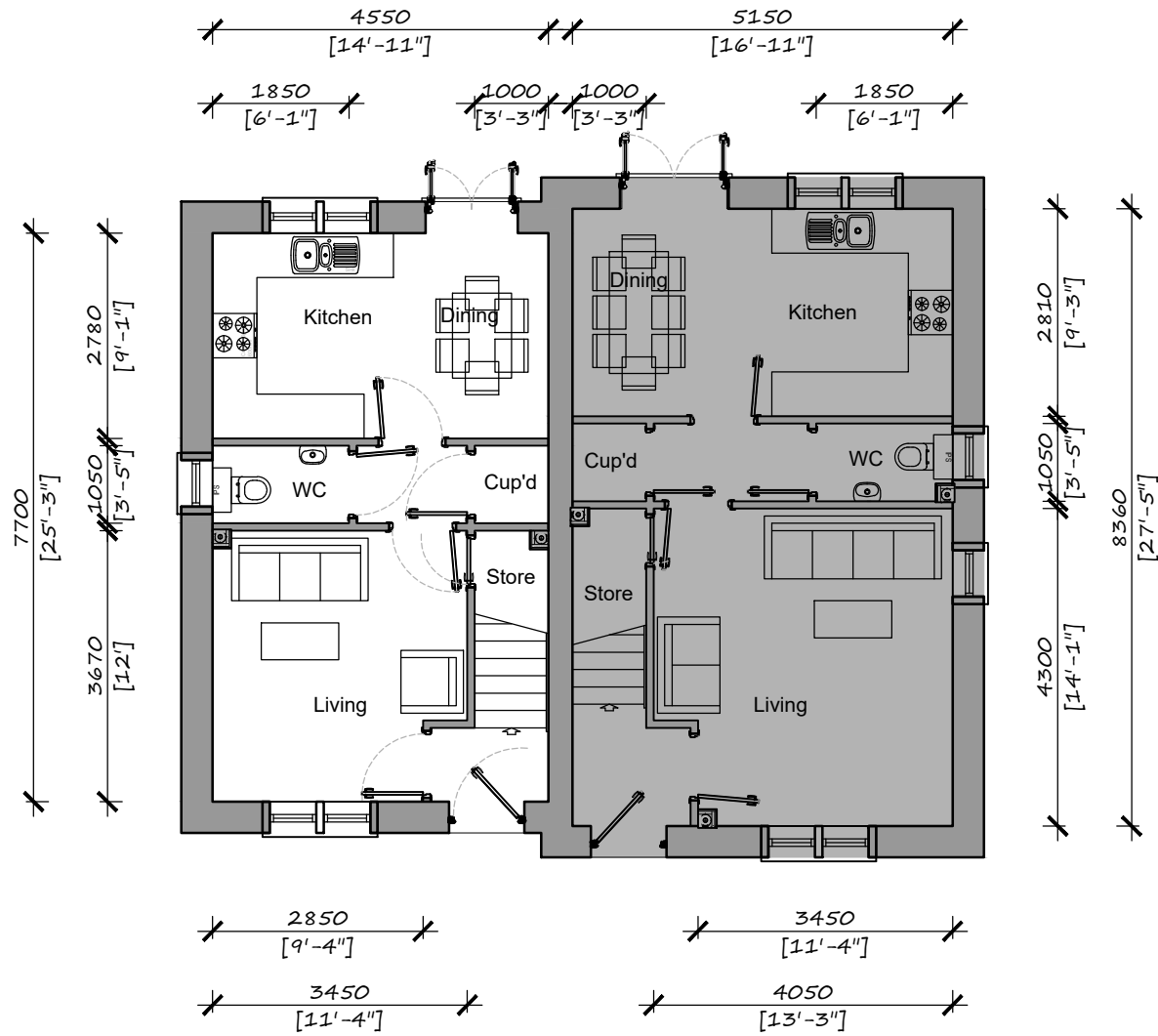
Plot 6 Ground Floor
