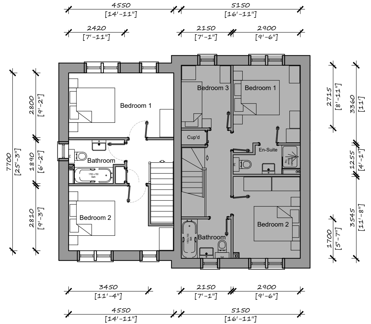
Plot 6 First Floor
